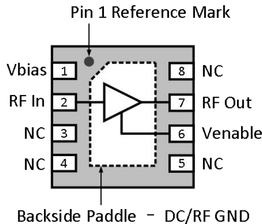
Figure2. Pin Assignments
